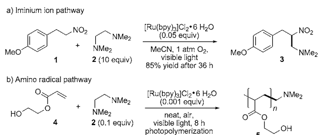
Scheme 2. Visible-light-promoted photocatalytic C–C bond cleavage of \text{Me}_2\text{NCH}_2\text{CH}_2\text{NMe}_2 . a) Formation of an iminium ion for aza-Henry reaction. b) Formation of an amino radical for photopolymerization.
