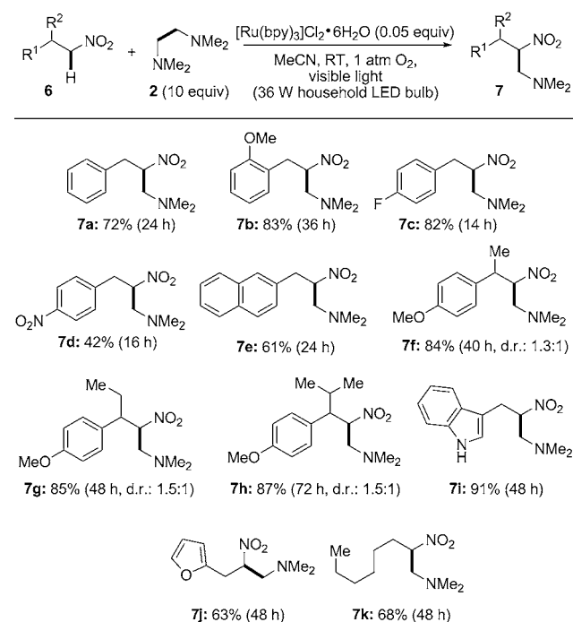
Scheme 3. Visible-light-promoted aza-Henry reactions by means of the photocatalytic C–C bond cleavage of \text{Me}_2\text{NCH}_2\text{CH}_2\text{NMe}_2 . Yields are of the isolated product.
