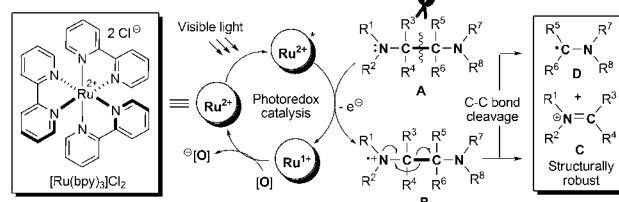
Scheme 1. Design concept for visible-light-promoted photocatalytic C–C bond cleavage of the substituted the 1,2-diamine A which leads to simultaneous generation of the structurally variable iminium ion C and amino radical D as reactive intermediates. [O] denotes an oxidant, and * denotes a photoexcited state.
